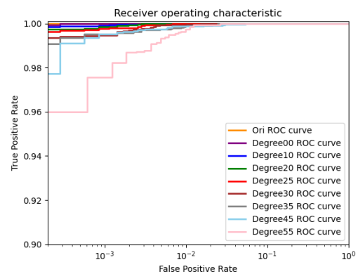
Figure 6: Fine-tune results on BIWI.
