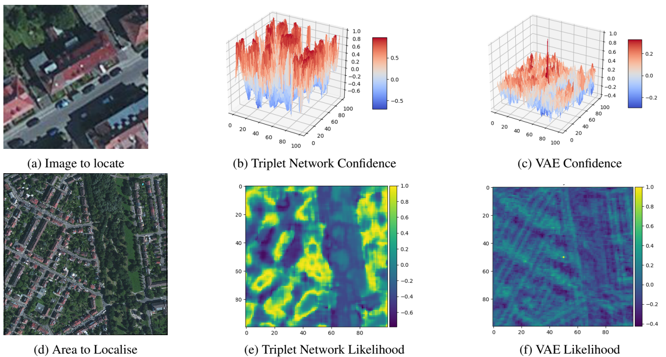
Figure 3: Localization likelihood calculated over a 500m 2 region. Samples were collected every 5m.
